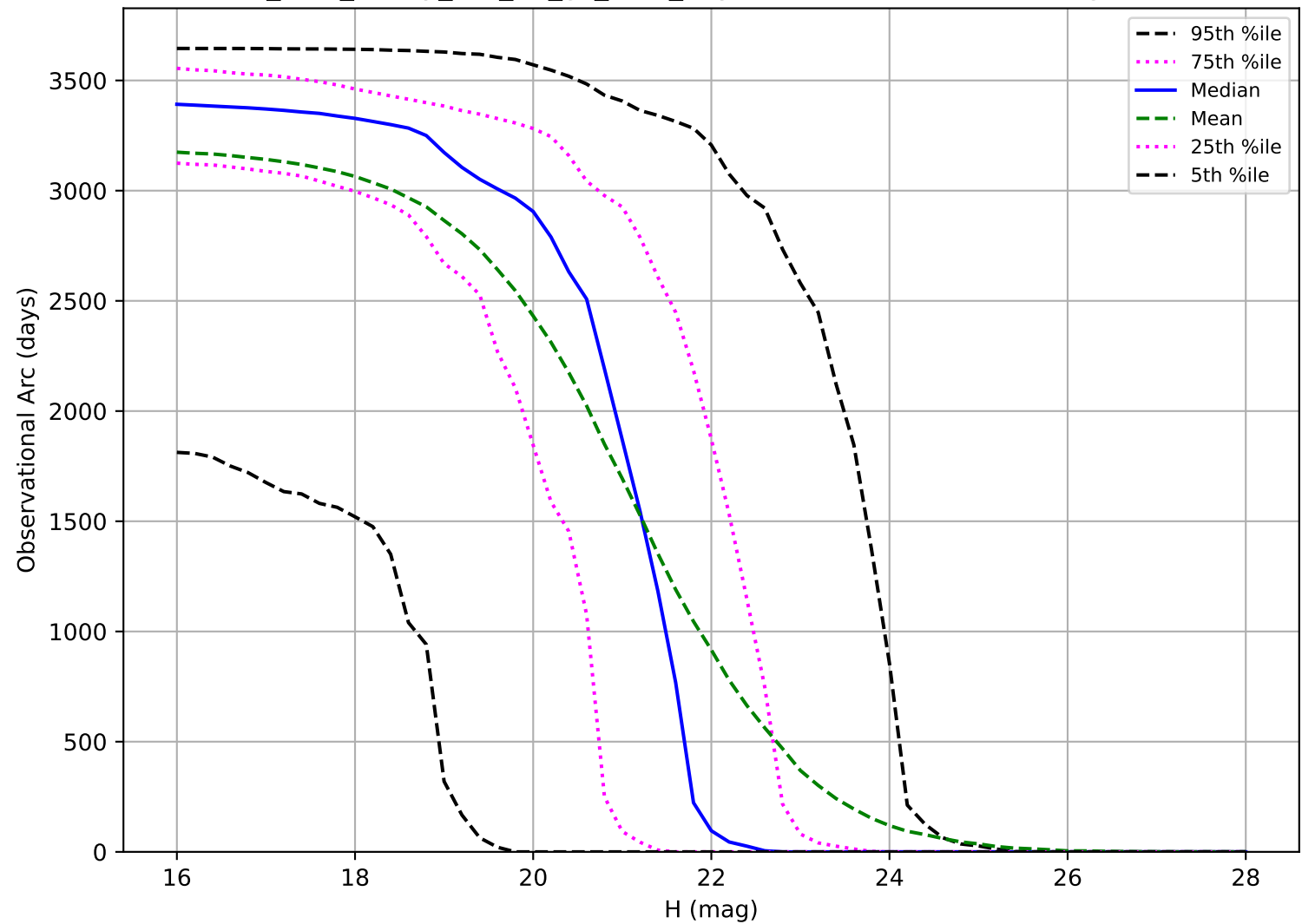
too_elab_heavy_r32_d3_gz_v3.4_10yrs: Observational Arc Length NEO
