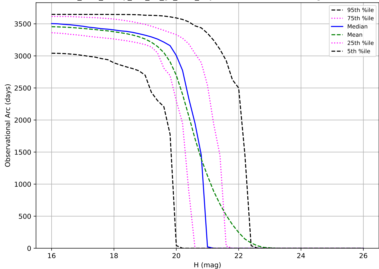
too_elab_heavy_r32_d3_gz_v3.4_10yrs: Observational Arc Length MBA
