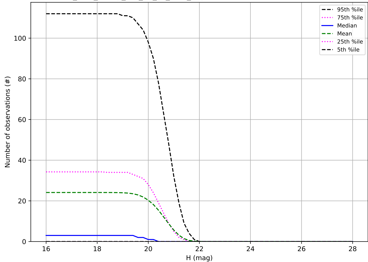
too_elab_heavy_r32_d3_gz_v3.4_10yrs: Number of observations Vatira
