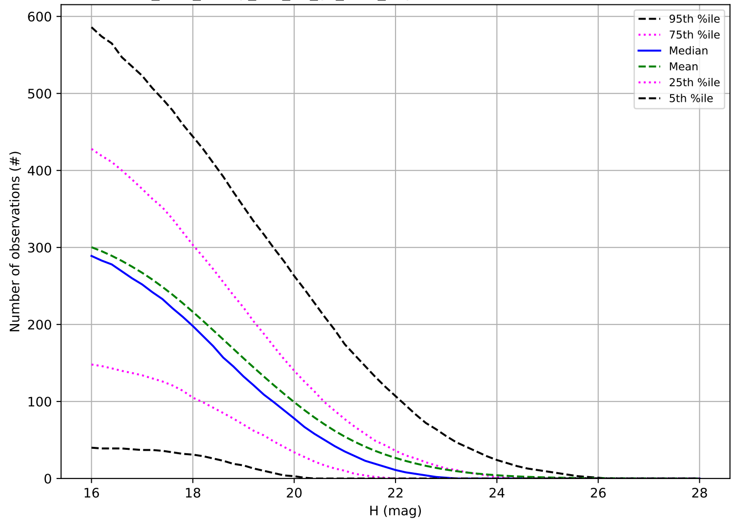
too_elab_heavy_r32_d3_gz_v3.4_10yrs: Number of observations PHA
