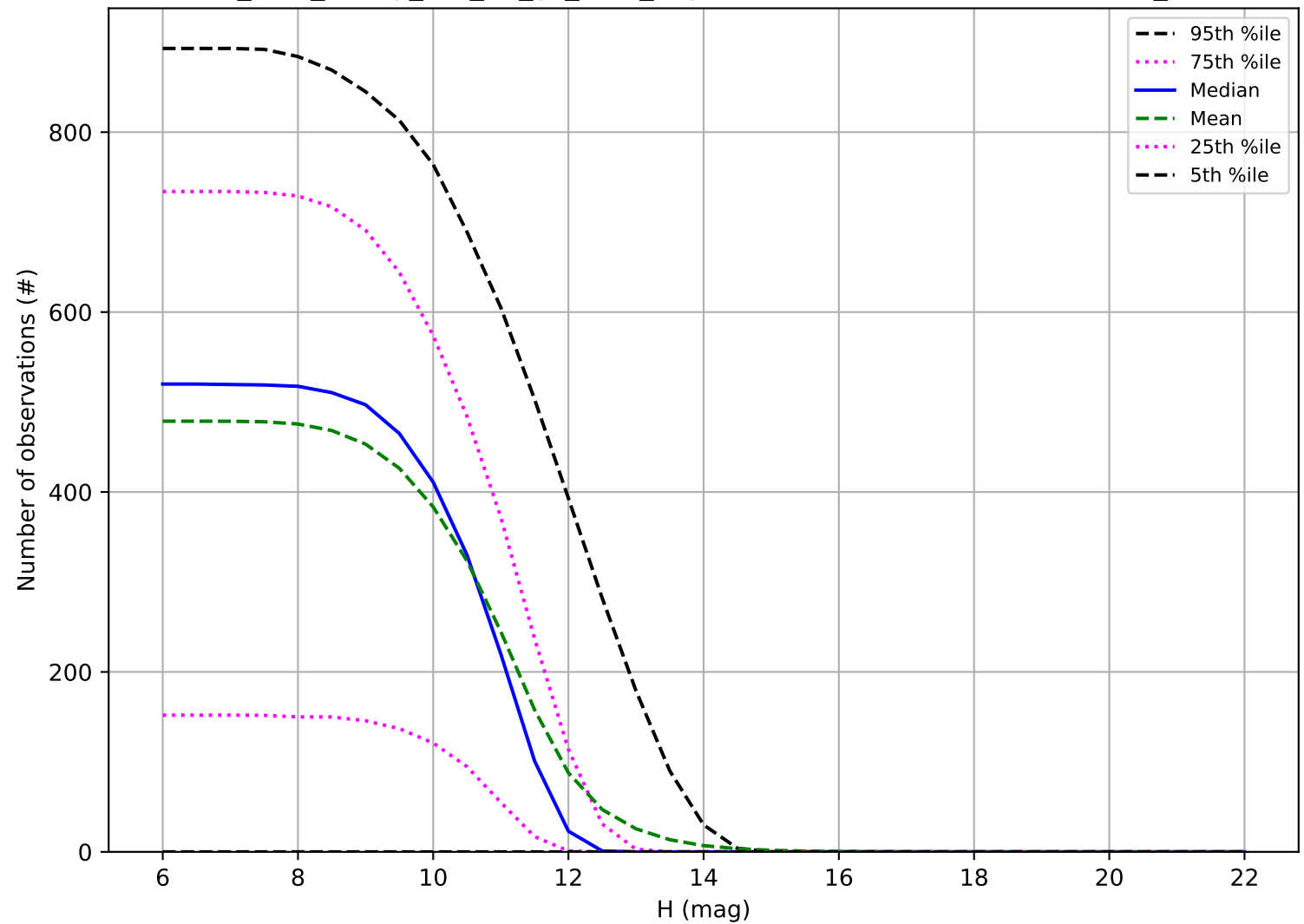
too_elab_heavy_r32_d3_gz_v3.4_10yrs: Number of observations OCC_r20
