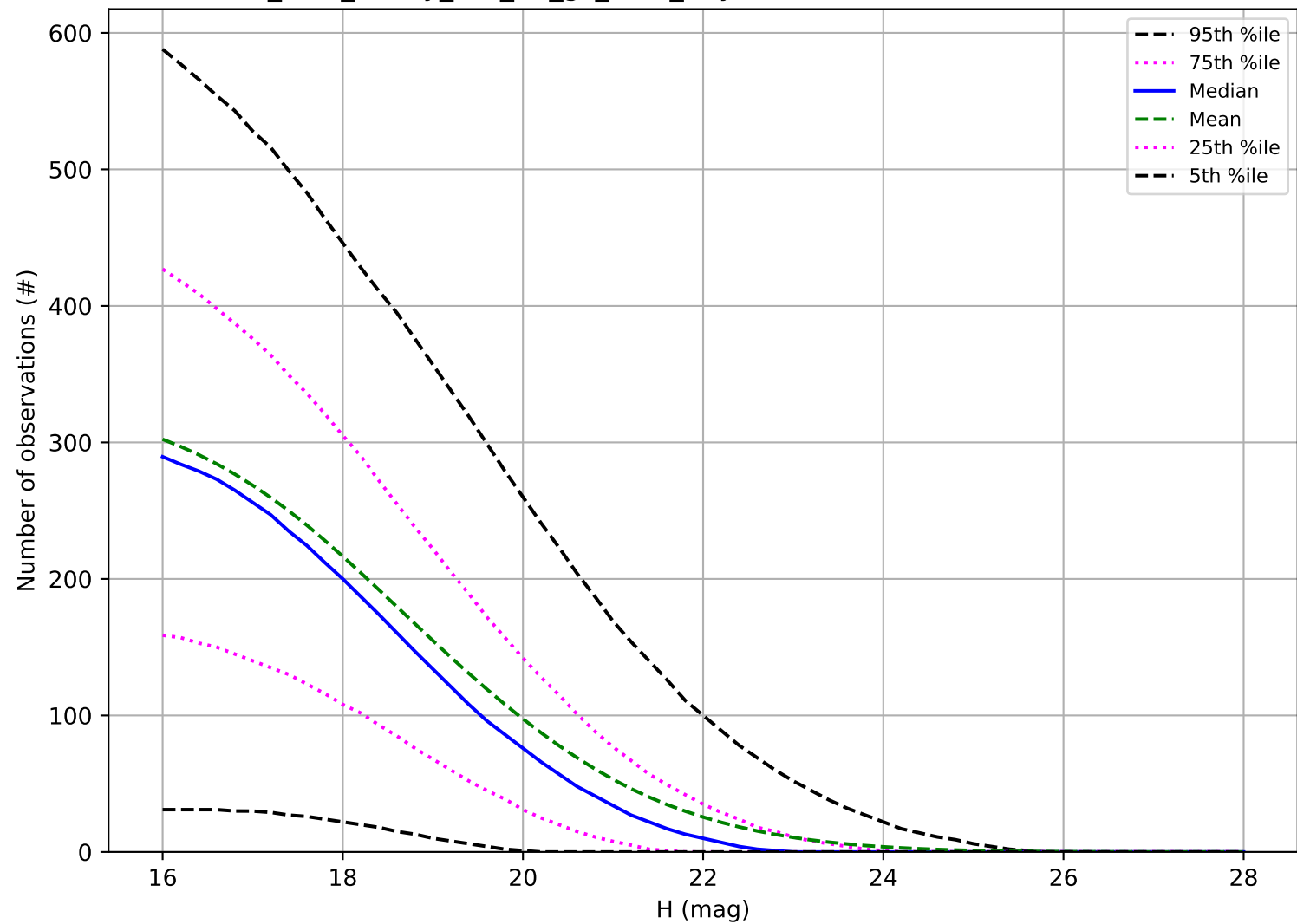
too_elab_heavy_r32_d3_gz_v3.4_10yrs: Number of observations NEO
