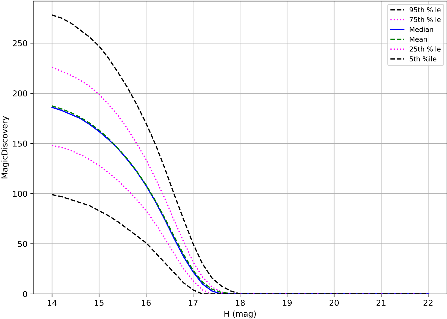
too_elab_heavy_r32_d3_gz_v3.4_10yrs: Trojan 6 detections in 60 nights detection loss
