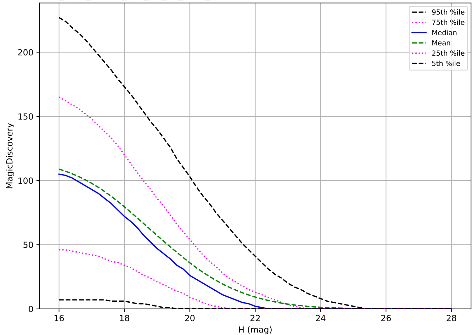
too_elab_heavy_r32_d3_gz_v3.4_10yrs: PHA 6 detections in 60 nights detection loss
