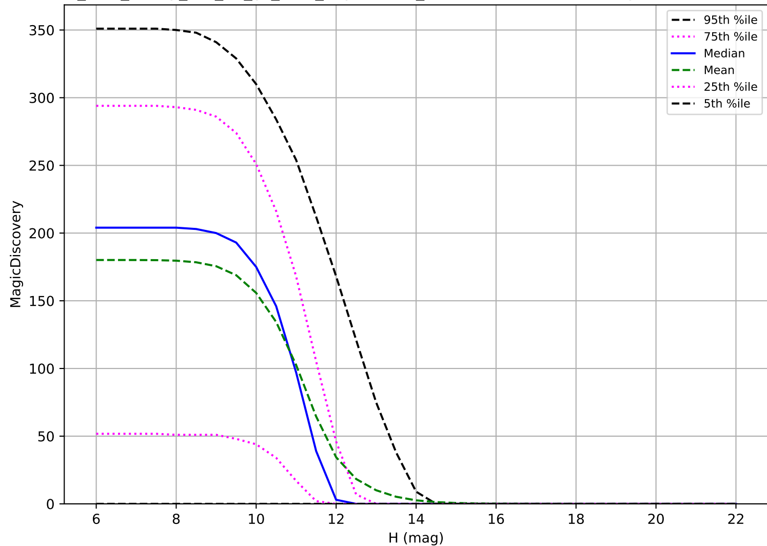
too_elab_heavy_r32_d3_gz_v3.4_10yrs: OCC_r20 6 detections in 60 nights detection loss
