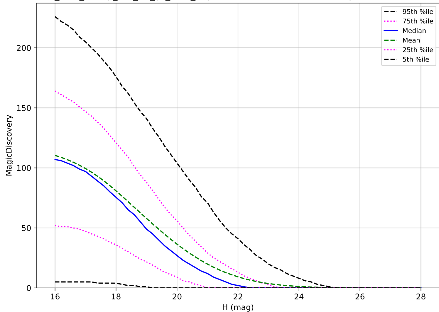
too_elab_heavy_r32_d3_gz_v3.4_10yrs: NEO 6 detections in 60 nights detection loss
