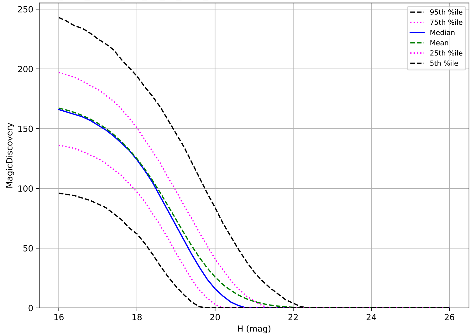
too_elab_heavy_r32_d3_gz_v3.4_10yrs: MBA 6 detections in 60 nights detection loss
