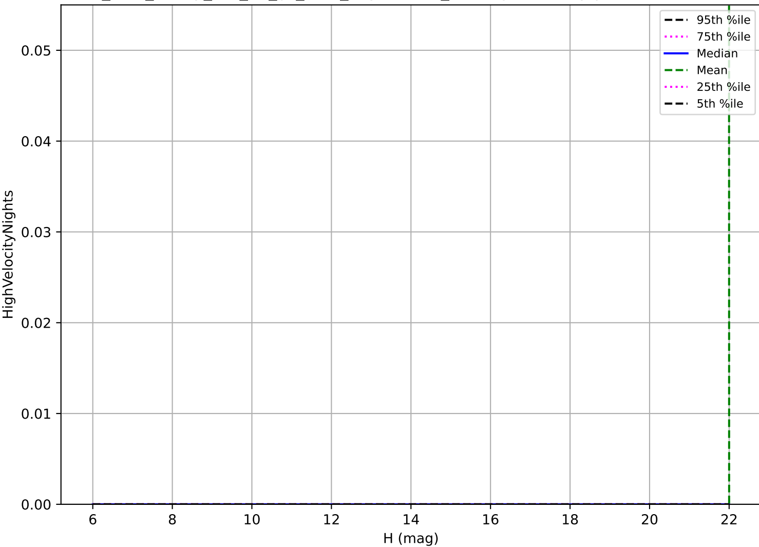
too_elab_heavy_r32_d3_gz_v3.4_10yrs: OCC_r20 High velocity pair detection loss
