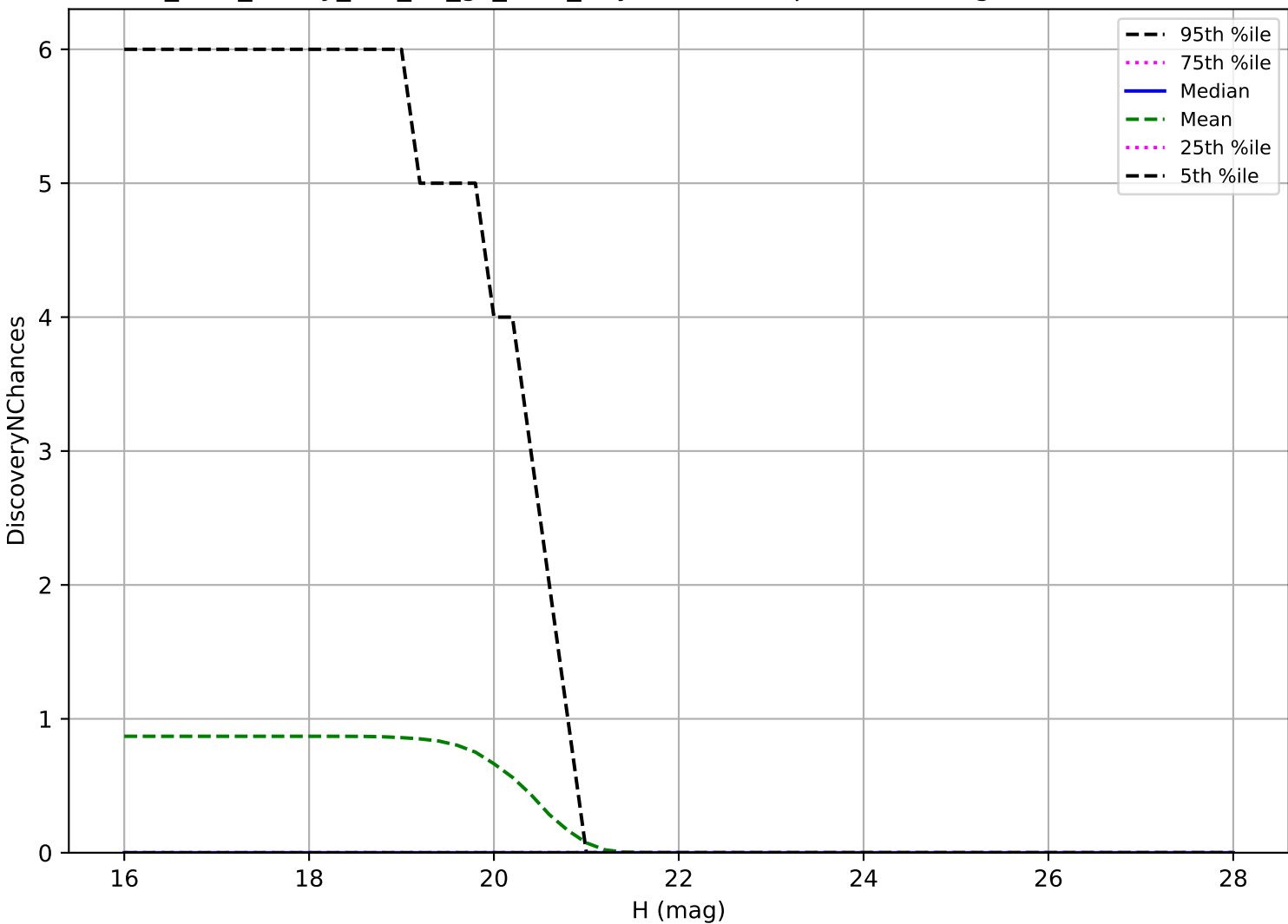
too_elab_heavy_r32_d3_gz_v3.4_10yrs: Vatira 3 pairs in 15 nights detection loss
