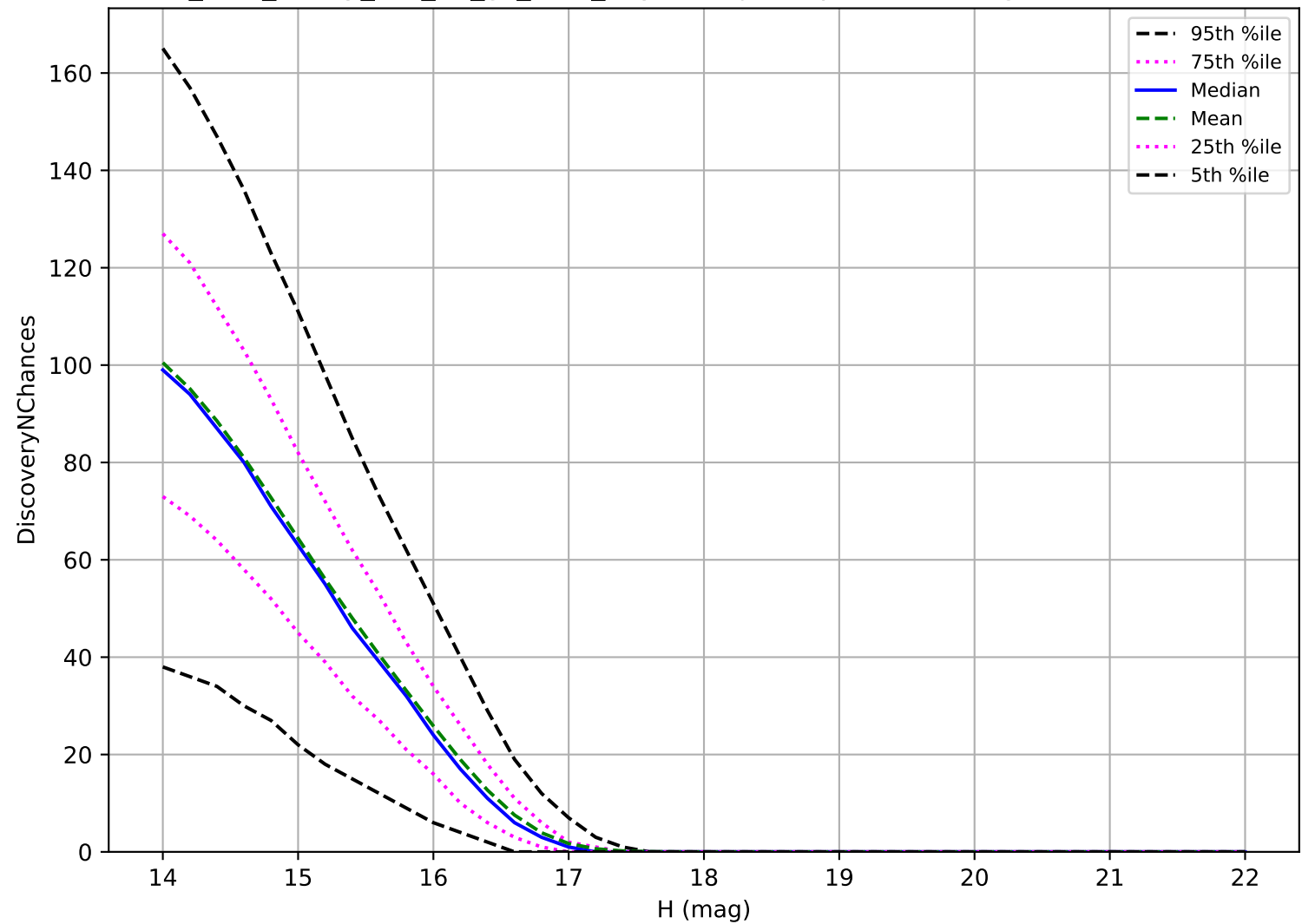
too_elab_heavy_r32_d3_gz_v3.4_10yrs: Trojan 3 pairs in 15 nights detection loss
