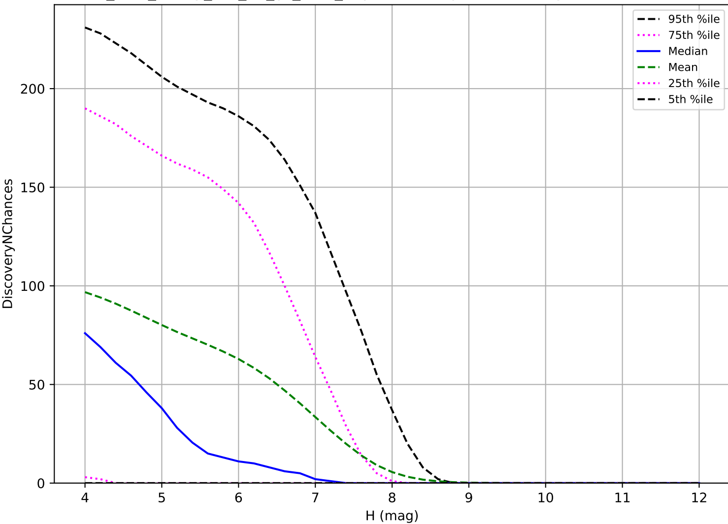
too_elab_heavy_r32_d3_gz_v3.4_10yrs: TNO 3 pairs in 15 nights detection loss
