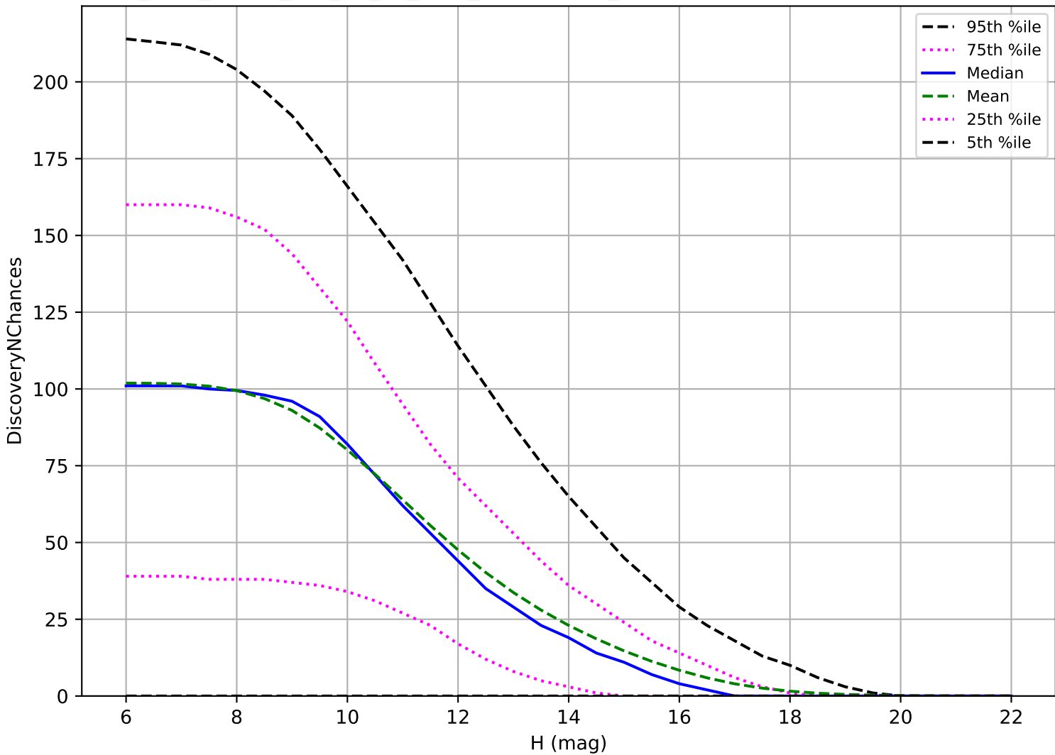
too_elab_heavy_r32_d3_gz_v3.4_10yrs: OCC_r5 3 pairs in 15 nights detection loss
