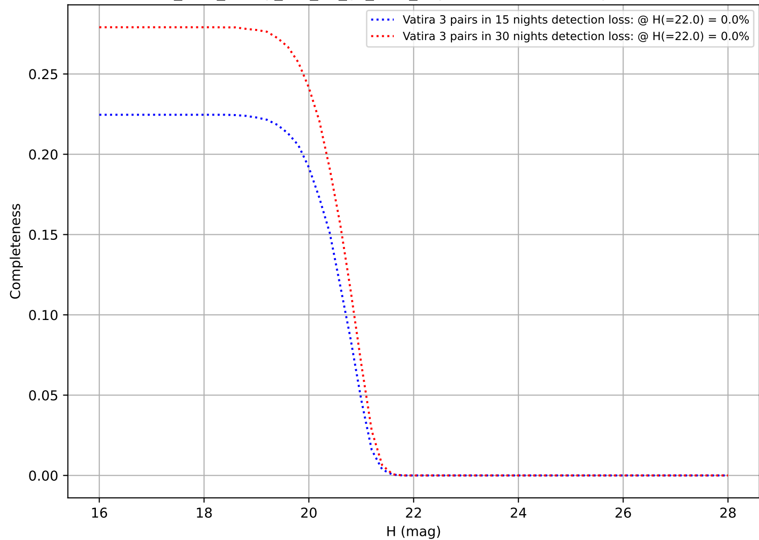
too_elab_heavy_r32_d3_gz_v3.4_10yrs: DifferentialCompleteness
