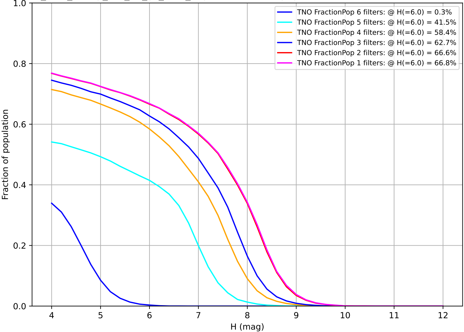
too_elab_heavy_r32_d3_gz_v3.4_10yrs: Fraction of population with colors in X filters TNO
