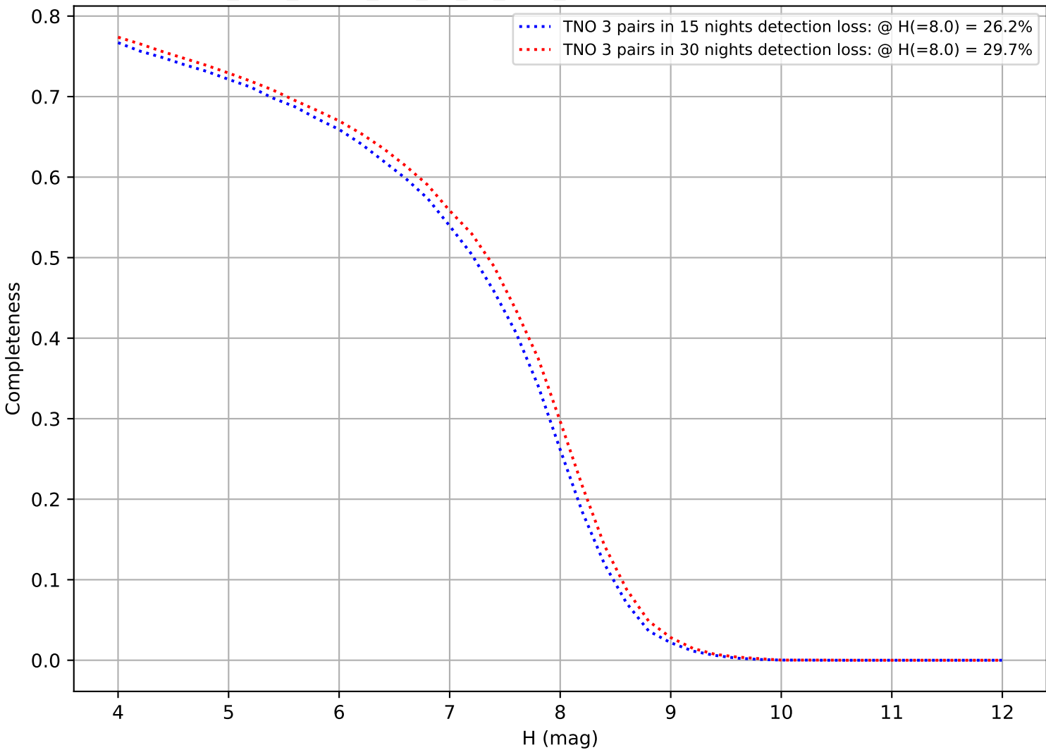
too_elab_heavy_r32_d3_gz_v3.4_10yrs: DifferentialCompleteness
