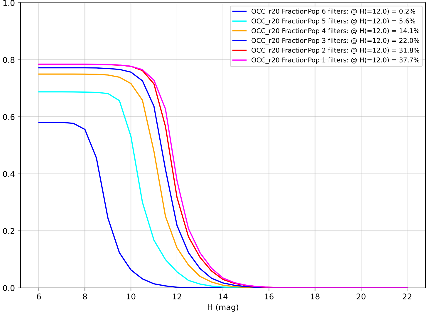
too_elab_heavy_r32_d3_gz_v3.4_10yrs: Fraction of population with colors in X filters OCC_r20
