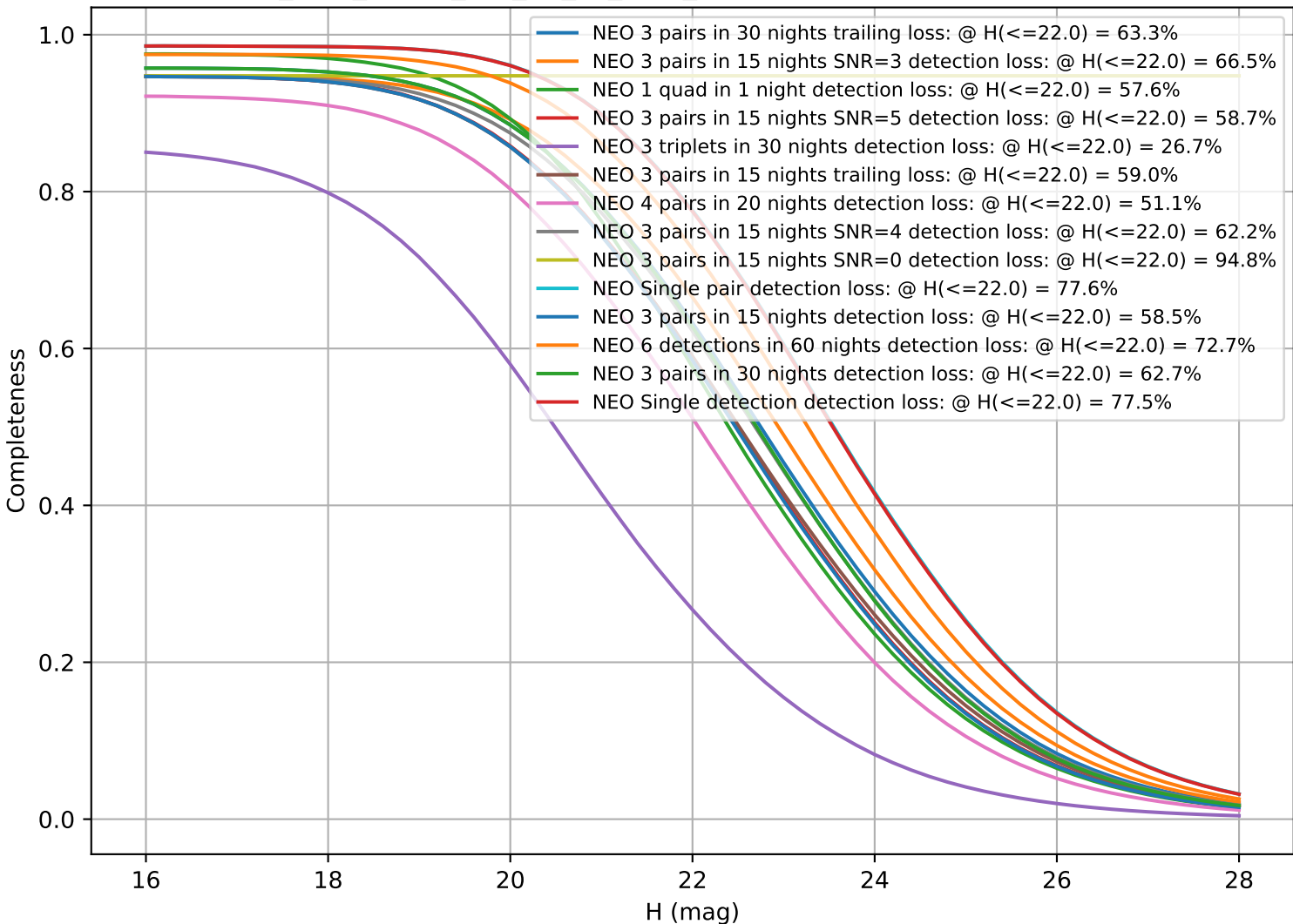
too_elab_heavy_r32_d3_gz_v3.4_10yrs: CumulativeCompleteness
