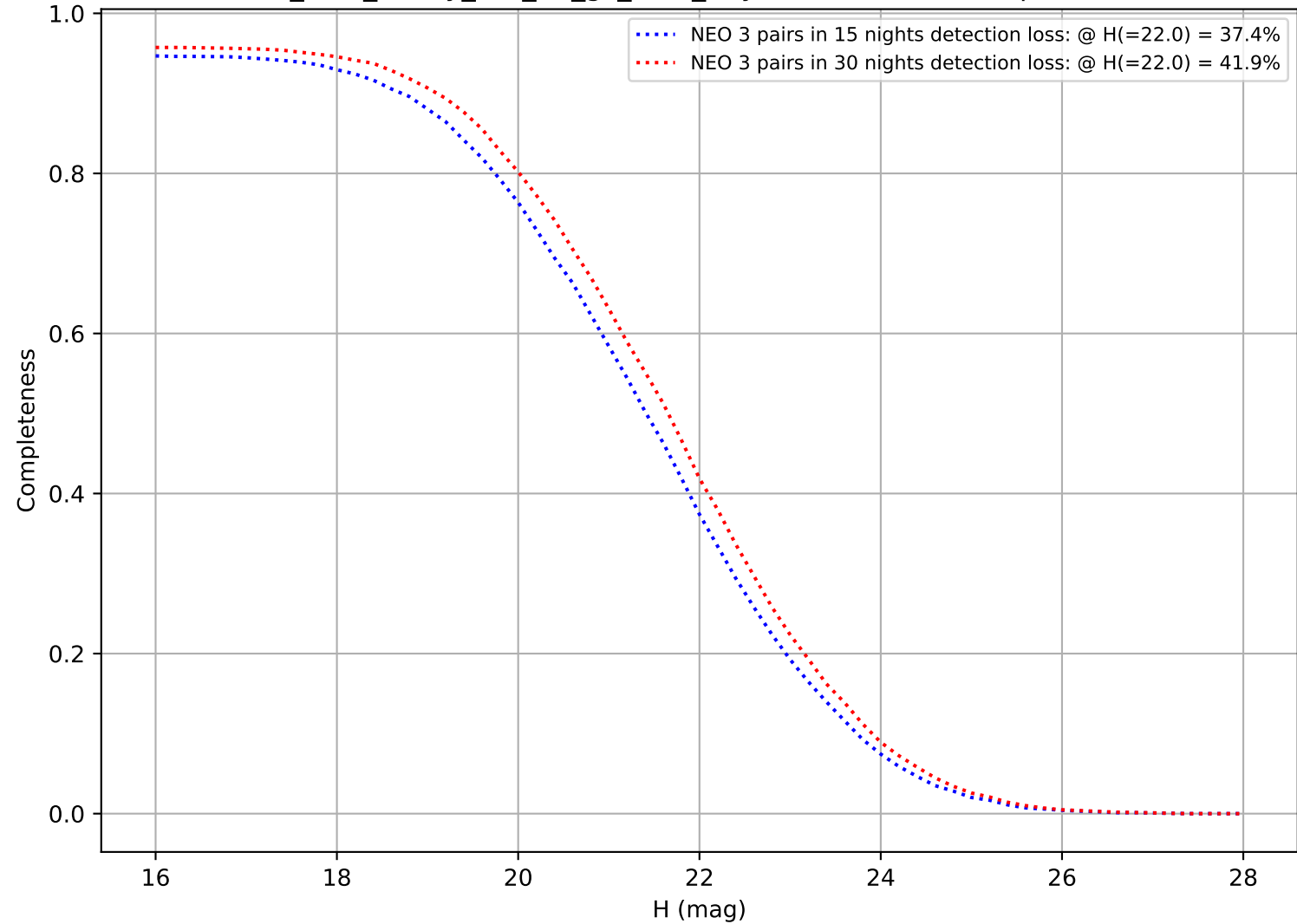
too_elab_heavy_r32_d3_gz_v3.4_10yrs: DifferentialCompleteness
