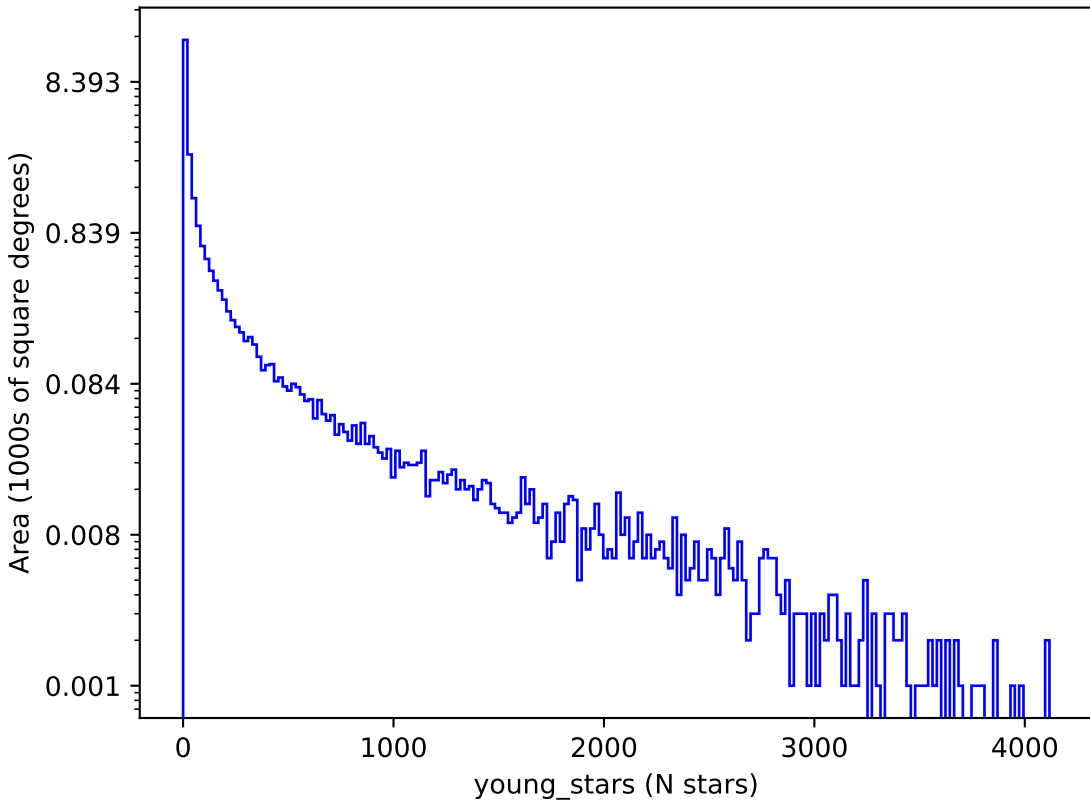
too_elab_heavy_r32_d3_gz_v3.4_10yrs : young_stars
