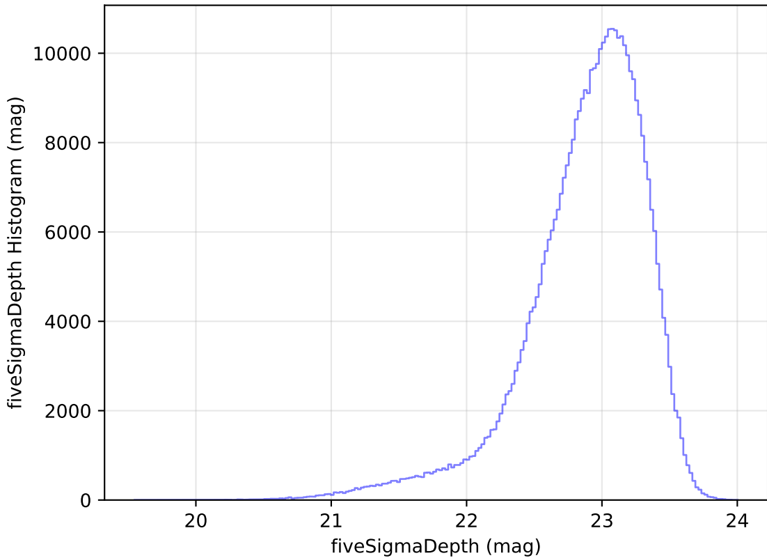
too_elab_heavy_r32_d3_gz_v3.4_10yrs z: fiveSigmaDepth Histogram
