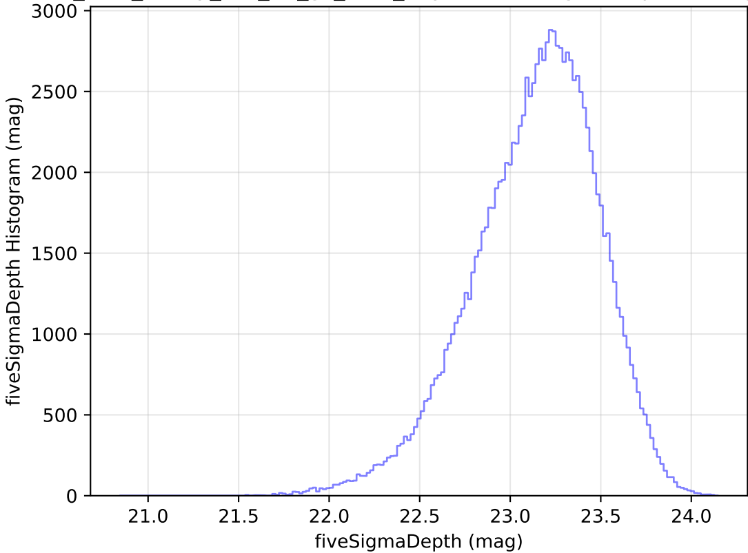
too_elab_heavy_r32_d3_gz_v3.4_10yrs u: fiveSigmaDepth Histogram
