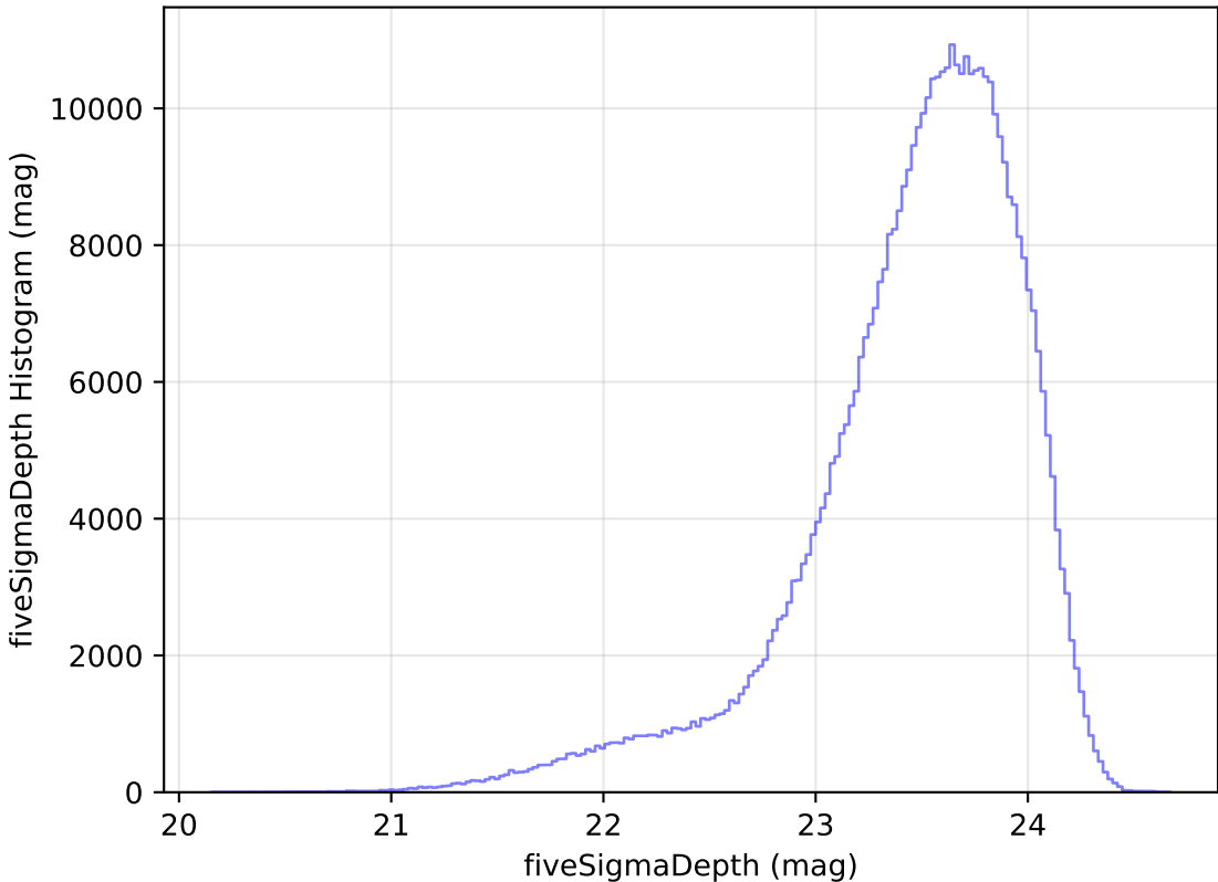
too_elab_heavy_r32_d3_gz_v3.4_10yrs i: fiveSigmaDepth Histogram
