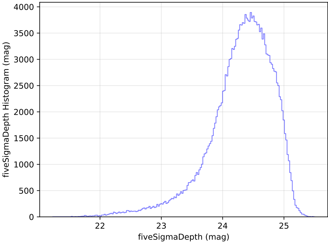
too_elab_heavy_r32_d3_gz_v3.4_10yrs g: fiveSigmaDepth Histogram
