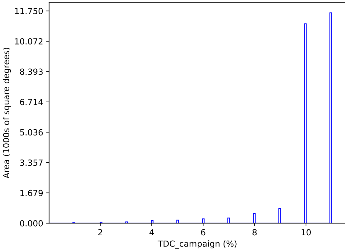
too_elab_heavy_r32_d3_gz_v3.4_10yrs : TDC_campaign
