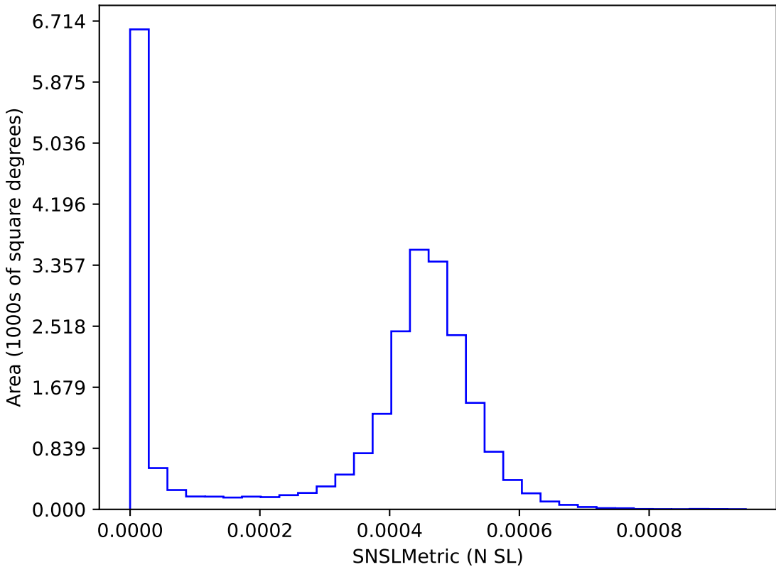
too_elab_heavy_r32_d3_gz_v3.4_10yrs : SNSLMetric
