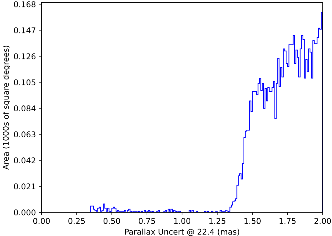
too_elab_heavy_r32_d3_gz_v3.4_10yrs : Parallax Uncert @ 22.4
