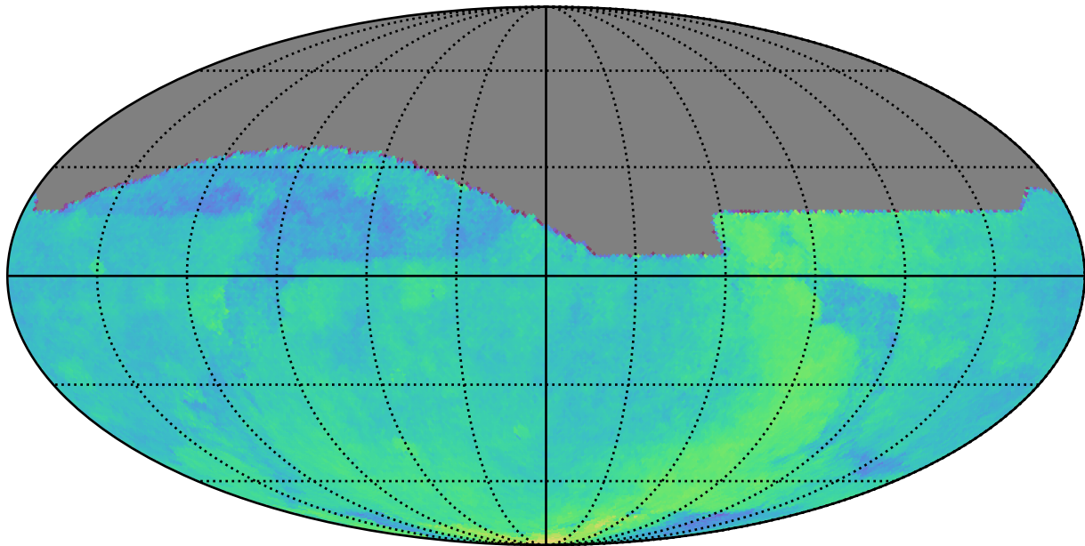
too_elab_heavy_r32_d3_gz_v3.4_10yrs : Parallax Coverage @ 22.4
