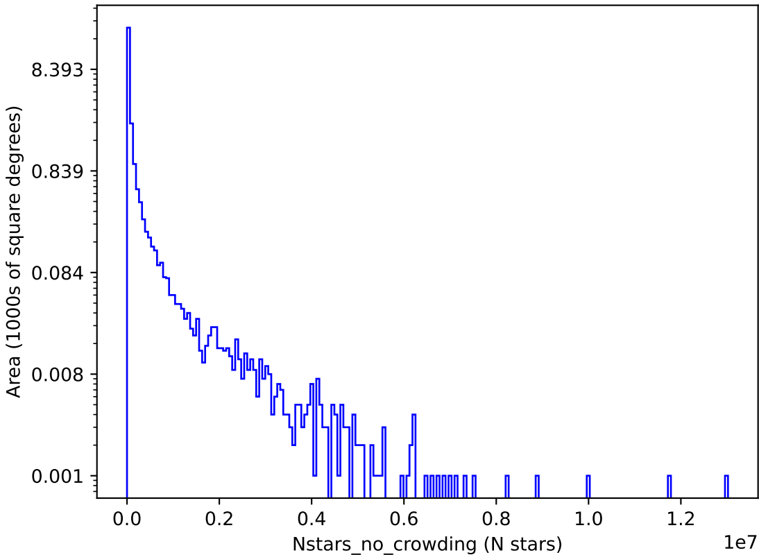
too_elab_heavy_r32_d3_gz_v3.4_10yrs g: Nstars_no_crowding
