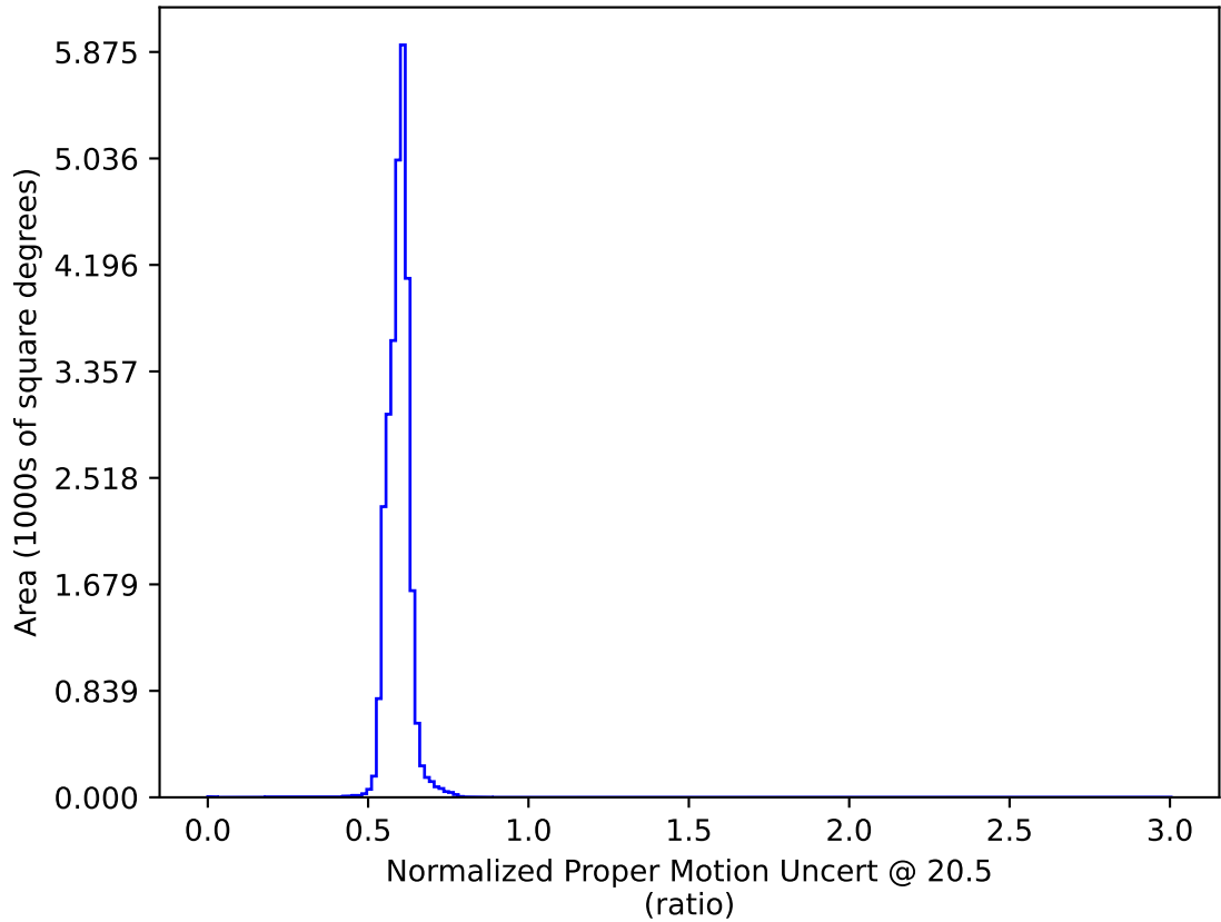
too_elab_heavy_r32_d3_gz_v3.4_10yrs : Normalized Proper Motion Uncert @ 20.5
