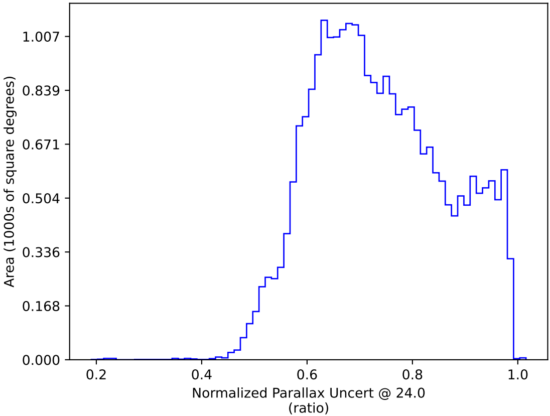
too_elab_heavy_r32_d3_gz_v3.4_10yrs : Normalized Parallax Uncert @ 24.0
