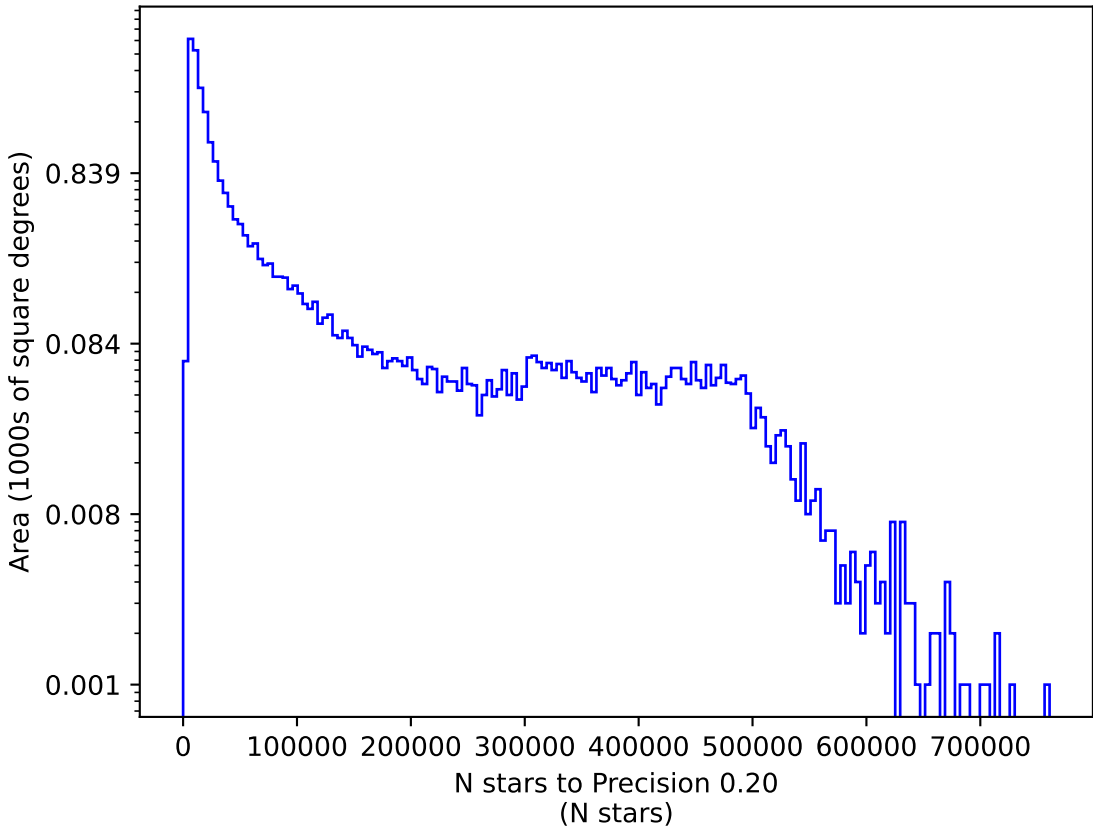
too_elab_heavy_r32_d3_gz_v3.4_10yrs r: N stars to Precision 0.20
