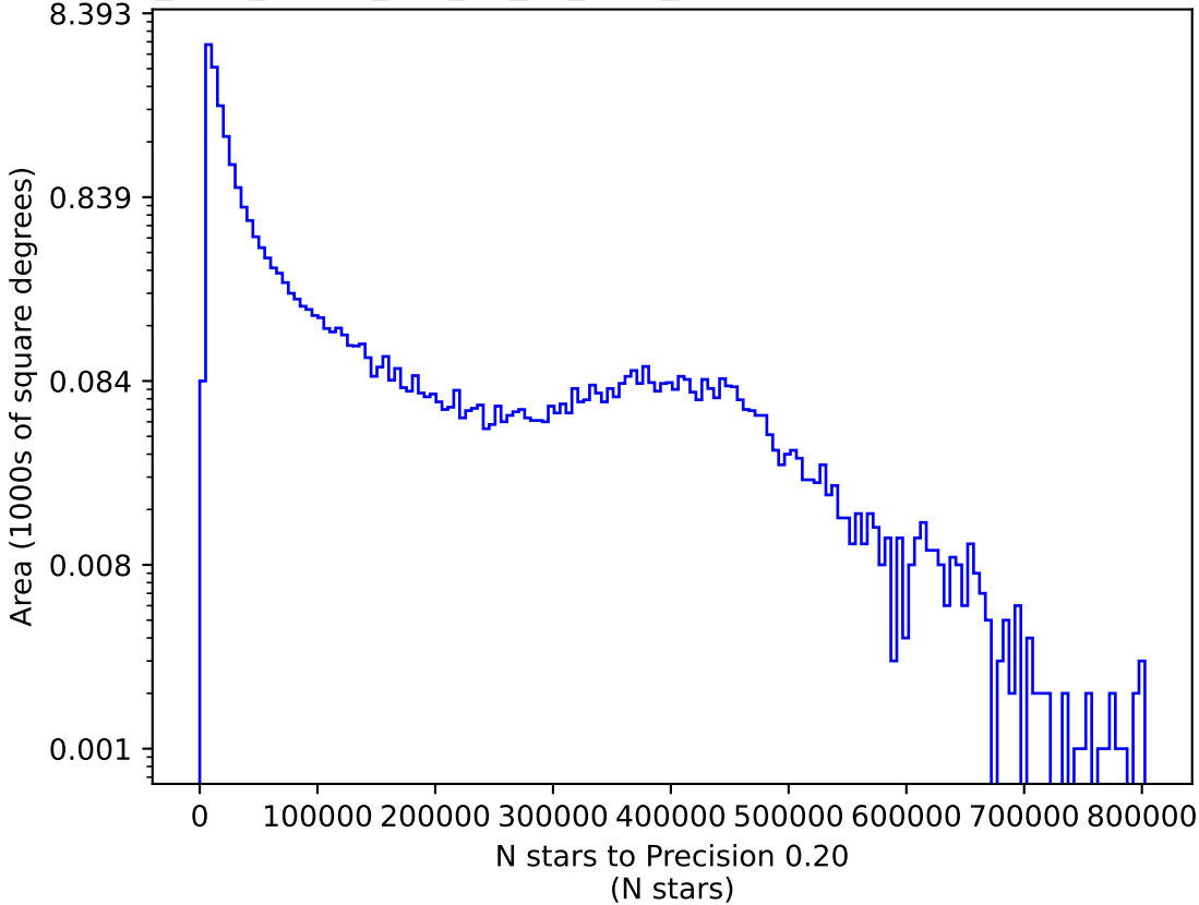
too_elab_heavy_r32_d3_gz_v3.4_10yrs i: N stars to Precision 0.20
