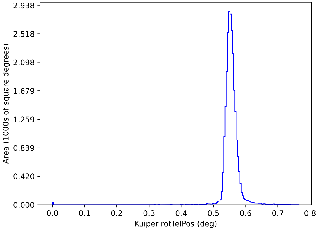
too_elab_heavy_r32_d3_gz_v3.4_10yrs y: Kuiper rotTelPos
