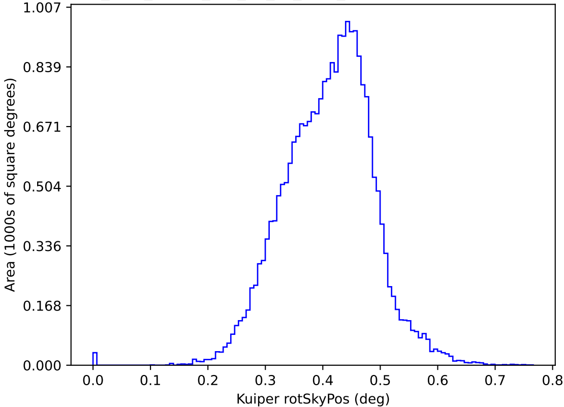
too_elab_heavy_r32_d3_gz_v3.4_10yrs y: Kuiper rotSkyPos
