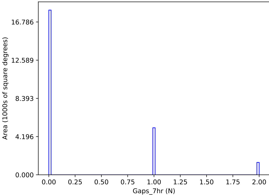
too_elab_heavy_r32_d3_gz_v3.4_10yrs y band: Gaps_7hr
