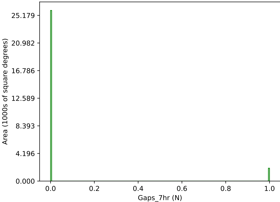
too_elab_heavy_r32_d3_gz_v3.4_10yrs g band: Gaps_7hr
