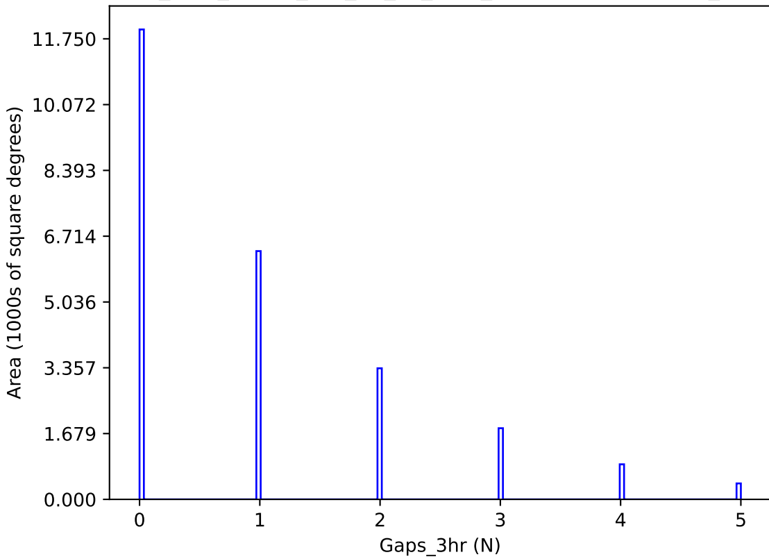
too_elab_heavy_r32_d3_gz_v3.4_10yrs y band: Gaps_3hr
