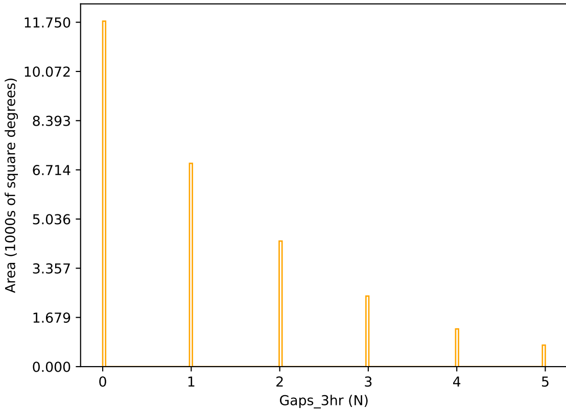
too_elab_heavy_r32_d3_gz_v3.4_10yrs r band: Gaps_3hr
