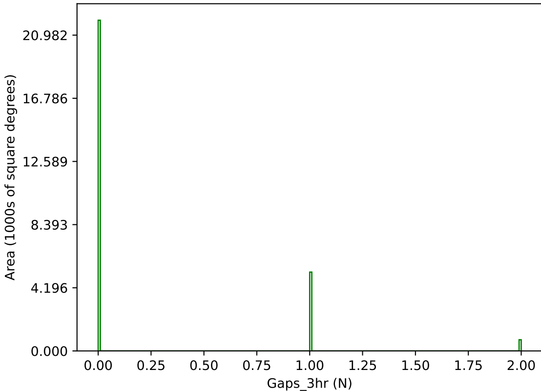
too_elab_heavy_r32_d3_gz_v3.4_10yrs g band: Gaps_3hr
