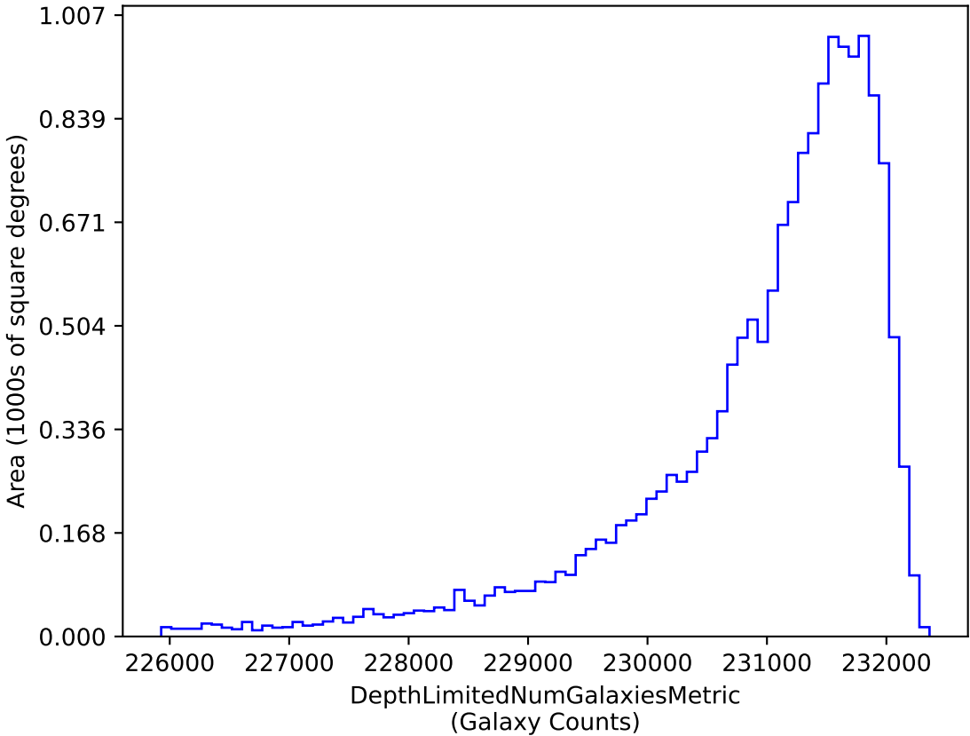
too_elab_heavy_r32_d3_gz_v3.4_10yrs i band galaxies non-DD: DepthLimitedNumGalaxiesMetric
