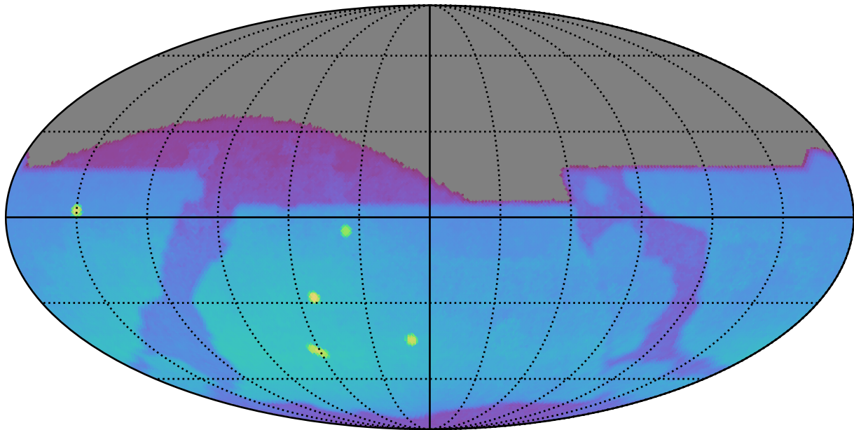
too_elab_heavy_r32_d3_gz_v3.4_10yrs : Brown Dwarf, L7
