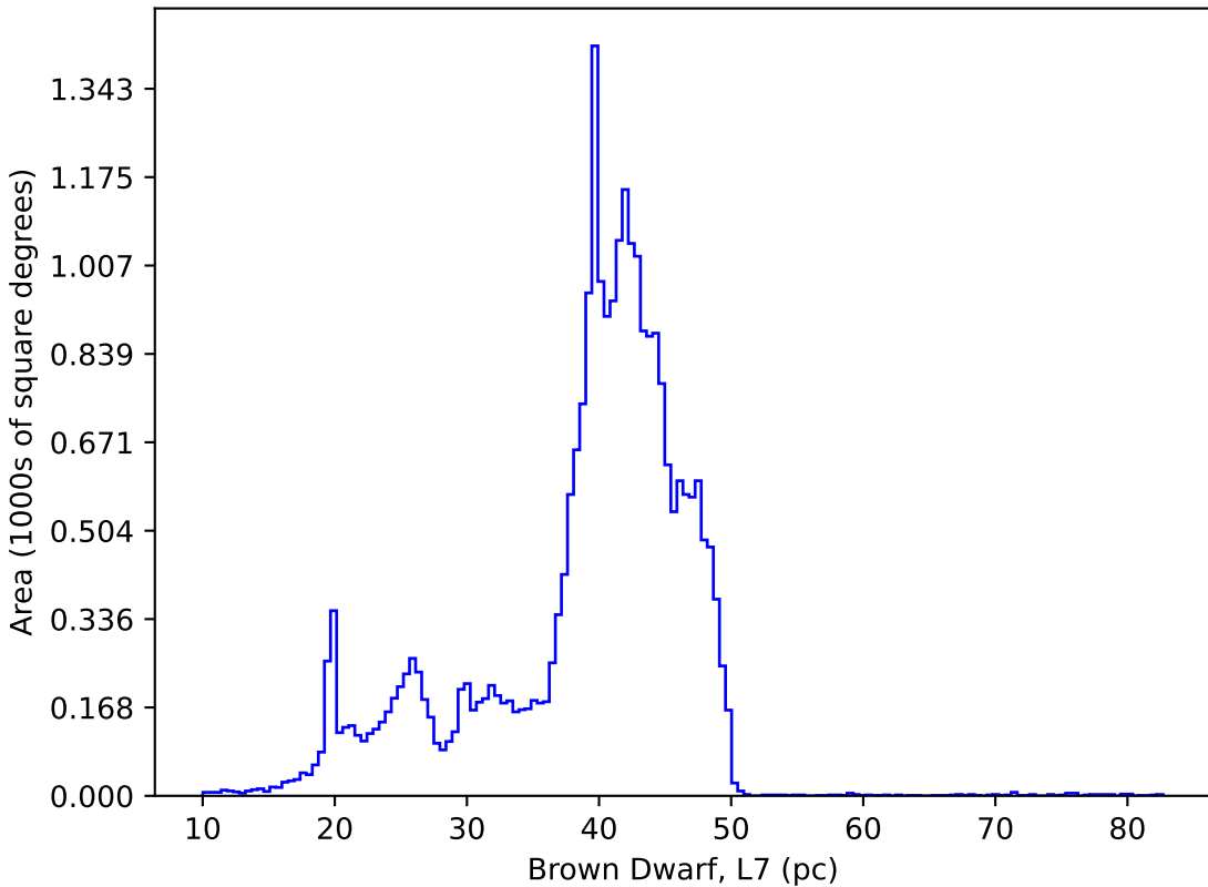
too_elab_heavy_r32_d3_gz_v3.4_10yrs : Brown Dwarf, L7
