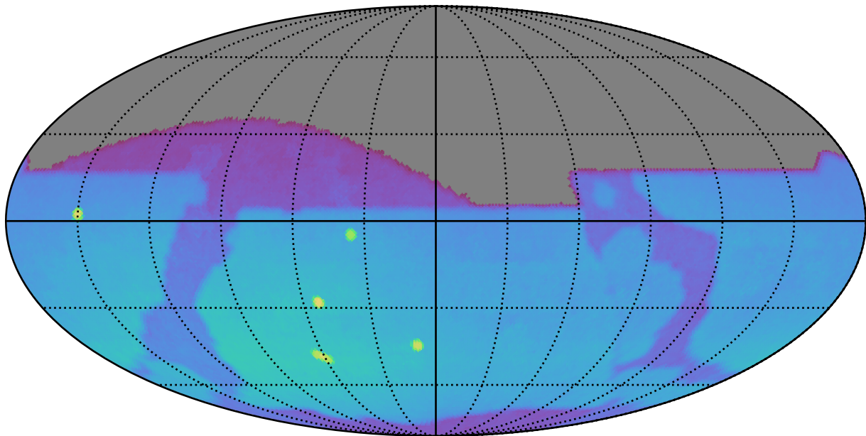
too_elab_heavy_r32_d3_gz_v3.4_10yrs : Brown Dwarf, L4
