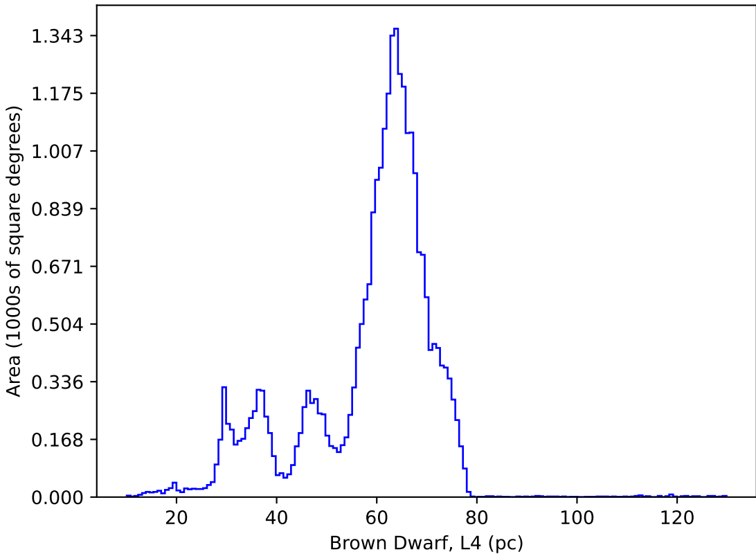
too_elab_heavy_r32_d3_gz_v3.4_10yrs : Brown Dwarf, L4
