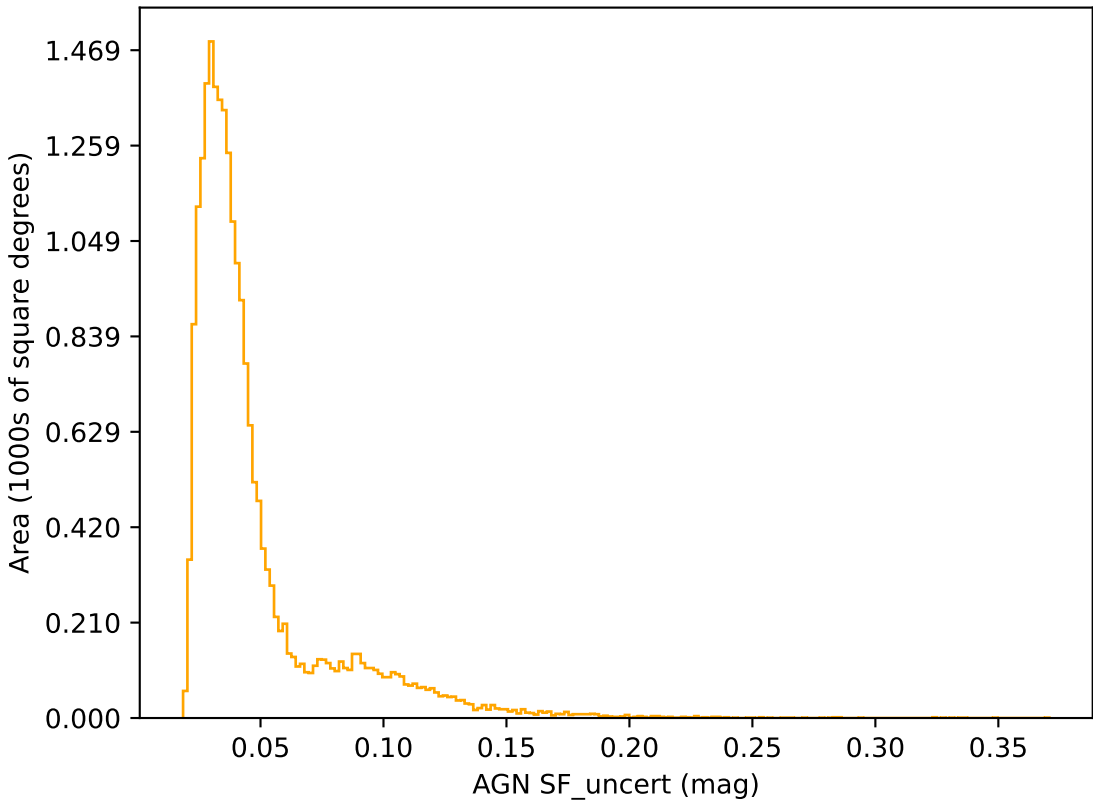
too_elab_heavy_r32_d3_gz_v3.4_10yrs r band: AGN SF_uncert
