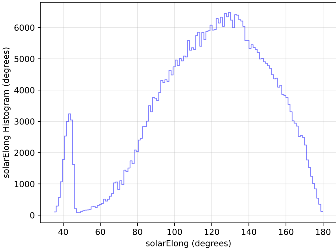
too_elab_heavy_r32_d3_gz_v3.4_10yrs WFD z band: solarElong Histogram
